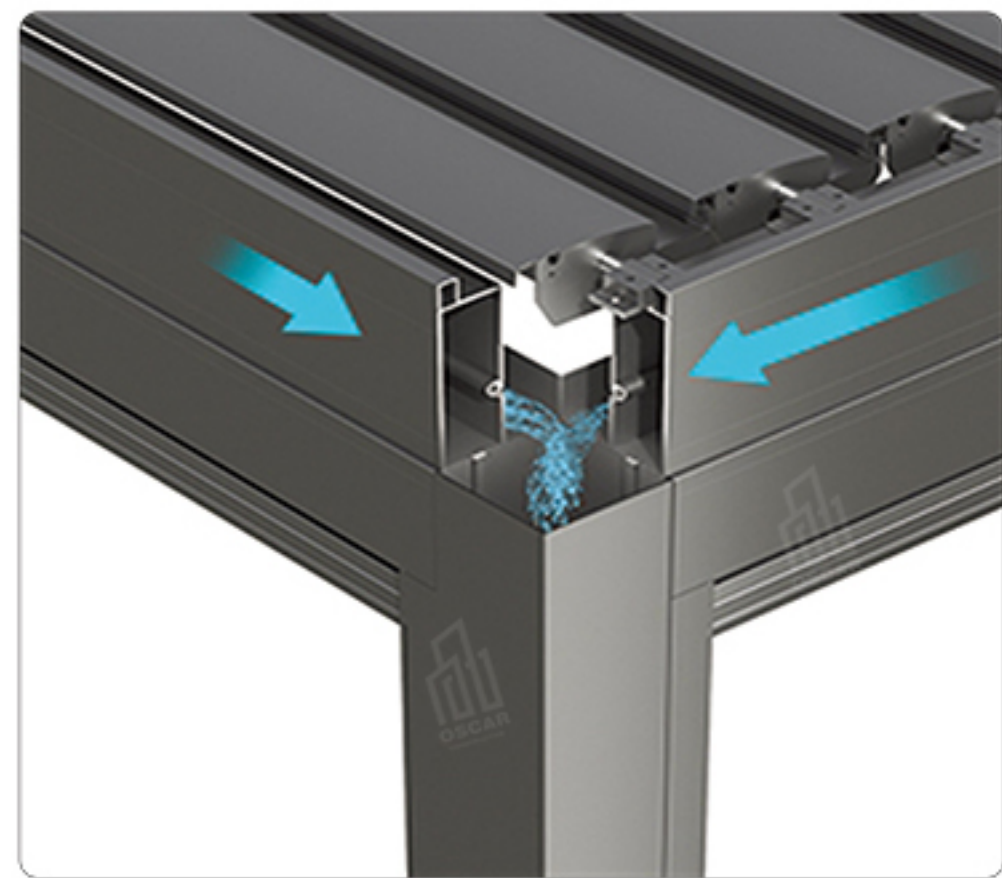
Rainwater direction
